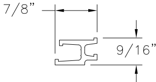
STILE REINFORCEMENT (10712) ALUMINUM 6005-T5
