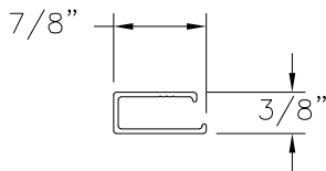
LOCK RAIL REINFORCEMENT (731A) ALUMINUM 6005-T5
