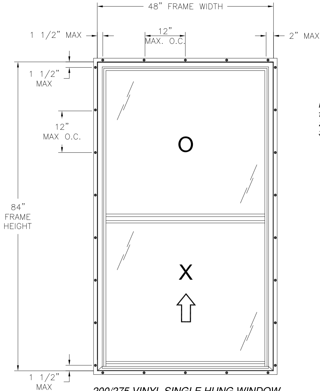
200/275 VINYL SINGLE HUNG WINDOW EXTERIOR VIEW
