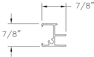
MEETING RAIL REINFORCEMENT (200A) ALUMINUM 6005-T5
